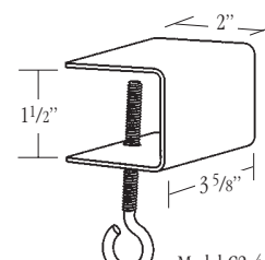
Model C2-4, Wide "C" Clamp
